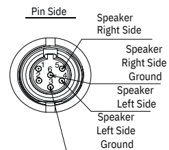
Pin Configuration for -112 Headset
