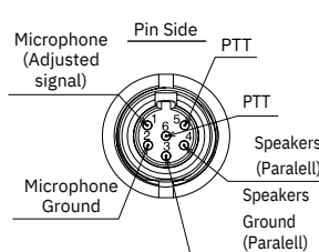
Pin Configuration for -111 Headset
