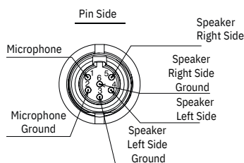
Pin Configuration for -110 Headset
